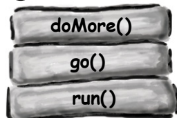
new thread
