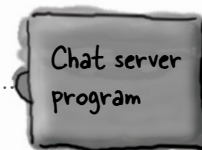
Server
