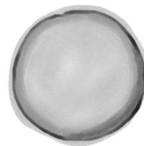
Dog object
